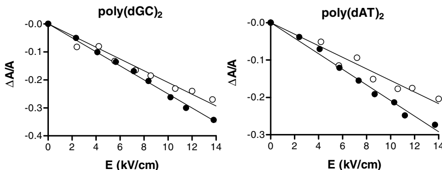
Figure 5. Variation of the reduced dichroism ( \Delta A/A ) for compound 5 bound to poly(dAT) 2 or poly(dGC) 2 , as a function of the electric field strength. \Delta A/A was measured at 360 nm and at a DNA/drug ratio of 20 in 1 mM sodium cacodylate buffer, pH 7.0 symbols (●) and (○) refer to the drug–polynucleotide complex and the polynucleotide alone, respectively.
