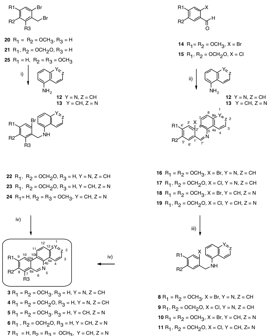
Scheme 1. Synthetic approach to the preparation of benzo[ c ][1,7] and [1,8] phenanthrolines derivatives. (i) neutral, alumina, toluene reflux, (ii) toluene reflux; (iii) \text{NaBH}_4 , MeOH, 0 °C; (iv) (1) LDA, THF, –78 °C; (2) air oxidation.
