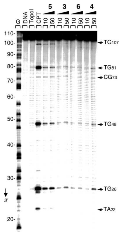
Figure 2. Cleavage of the 117-mer DNA fragment by topoisomerase I in the presence of the benzo[c]phenanthrolines 3–6 . The 3'-end labeled fragment (DNA) was incubated in the absence (lane TopoI) or presence of the alkaloids at 10 or 50 \mu M. Camptothecin (CPT) was used at 20 \mu M. Topoisomerase I cleavage reactions were analyzed on a 8% denaturing polyacrylamide gel. Numbers at the side of the gels show the nucleotide positions, determined with reference to the guanine track labeled G. The nucleotide positions and sequences of the main cleavage sites are indicated.
