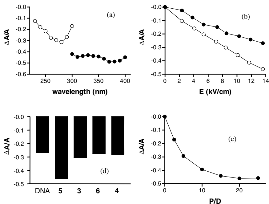
Figure 4. ELD data for the binding to DNA. Dependence of the reduced dichroism \Delta A/A on (a) the wavelength, (b) the electric field strength and (c) the DNA–drug ratio ( P/D ) for (●) compound 5 bound to calf thymus DNA and (○) DNA alone. Conditions: (a) 13.6 kV/cm, P/D=20 (200 \mu\text{M} calf thymus DNA, 10 \mu\text{M} drug), (b) 360 nm, P/D=20 for the DNA–drug complexes and 260 nm for the DNA alone (c) 13.6 kV/cm, 360 nm, in 1 mM sodium cacodylate buffer, pH 7.0. The histograms in panel (d) compare the reduced dichroism values ( \Delta A/A ) measured with DNA at 260 nm and the different drug–DNA complexes at 360 nm.
