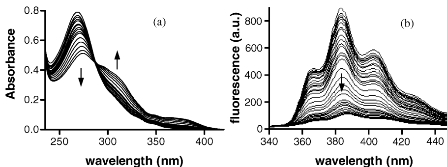
Figure 3. DNA titrations of 5 measured by (a) absorption and (b) fluorescence spectroscopy. To 1 mL of drug solution at (a) 20 \mu\text{M} or (b) 2.5 \mu\text{M} were added aliquots of a concentrated calf thymus DNA solution. The phosphate–DNA/drug ratio increased from 0 to 20 (top to bottom curves at (a) 270 nm or (b) 390 nm). For the fluorescence measurement, the excitation was set at 300 nm. Spectra were recorded in 1 mM sodium cacodylate buffer, pH 7.0.
