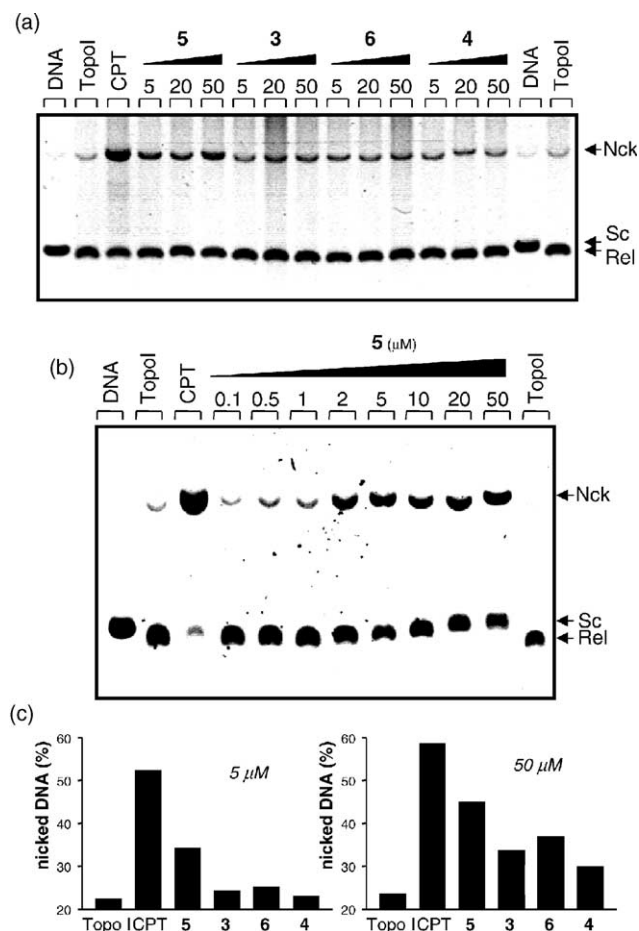
Figure 1. Topoisomerase I inhibition. (a) Effect of benzo[c]phenanthrolines 3–6 on the relaxation of plasmid DNA by topoisomerase I. Gel (b) shows the concentration-dependent effect of 5 tested at 0.1–50 \mu M, compared to CPT at 20 \mu M. Native supercoiled pLAZ3 DNA (0.3 \mu g) (lane DNA) was incubated with 4 units topoisomerase I in the absence (lane TopoI) or presence of drug at the indicated concentration ( \mu M). Reactions were stopped with sodium dodecylsulfate and treatment with proteinase K. DNA samples were separated by electrophoresis on 1% agarose gels containing ethidium (1 \mu g/mL) and then photographed under UV light. Nck, nicked; Rel, relaxed; Sc, supercoiled DNA. (c) Comparison of the extent of topoisomerase I-mediated DNA cleavage measured with 3–6 or CPT. The histogram shows the formation of nicked DNA (form II, %) for each compound. Band intensities from three gels such as the one shown in panel (a) were compiled for the quantitative analysis.
